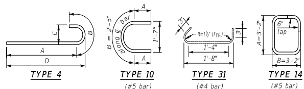
Reinforcement Details
